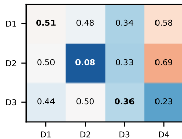
MSP
