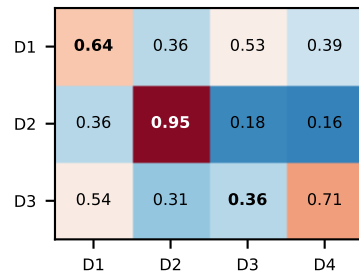
AHSD stress
