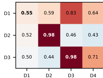
XGBoost
