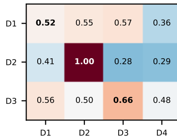
P(attack)†
