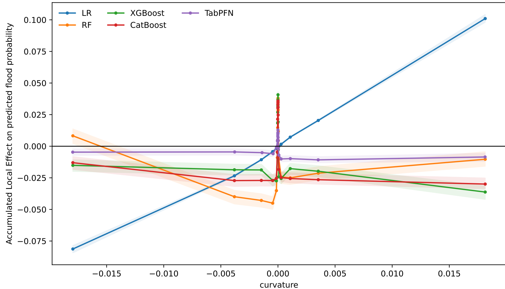
ALE comparison across five models — curvature
