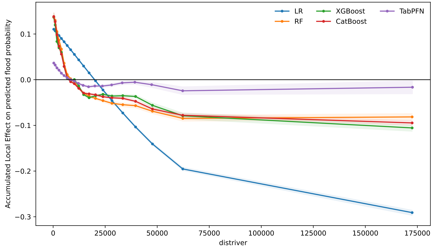
ALE comparison across five models — distriver
