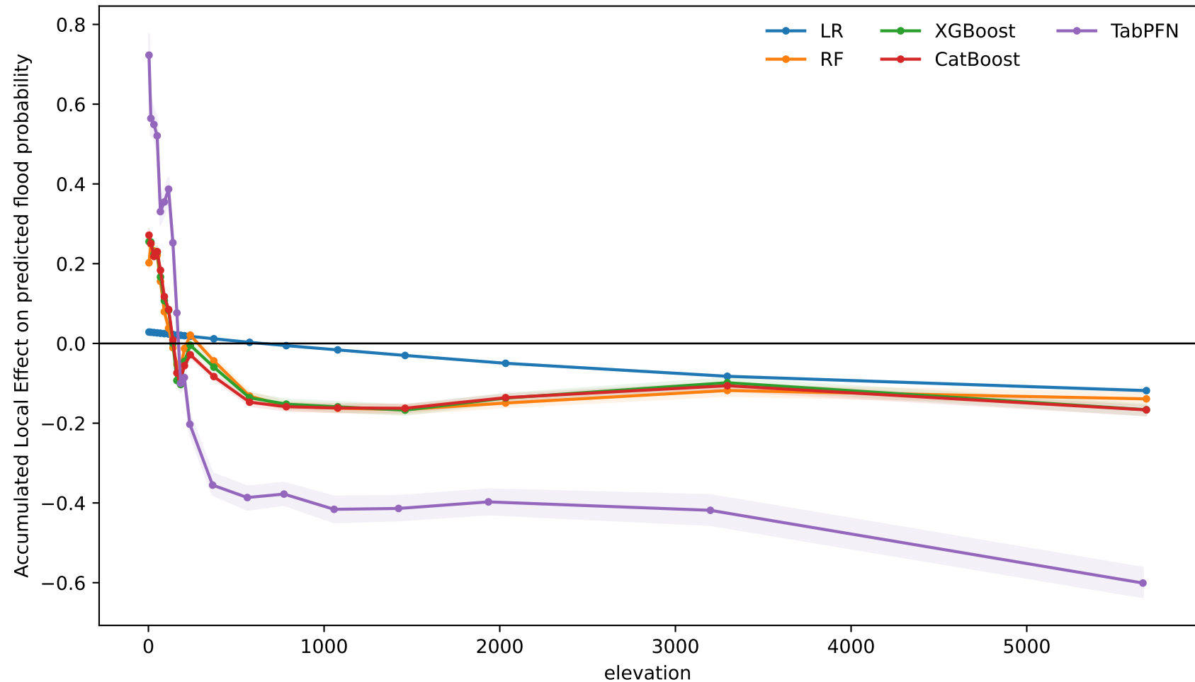
ALE comparison across five models — elevation
