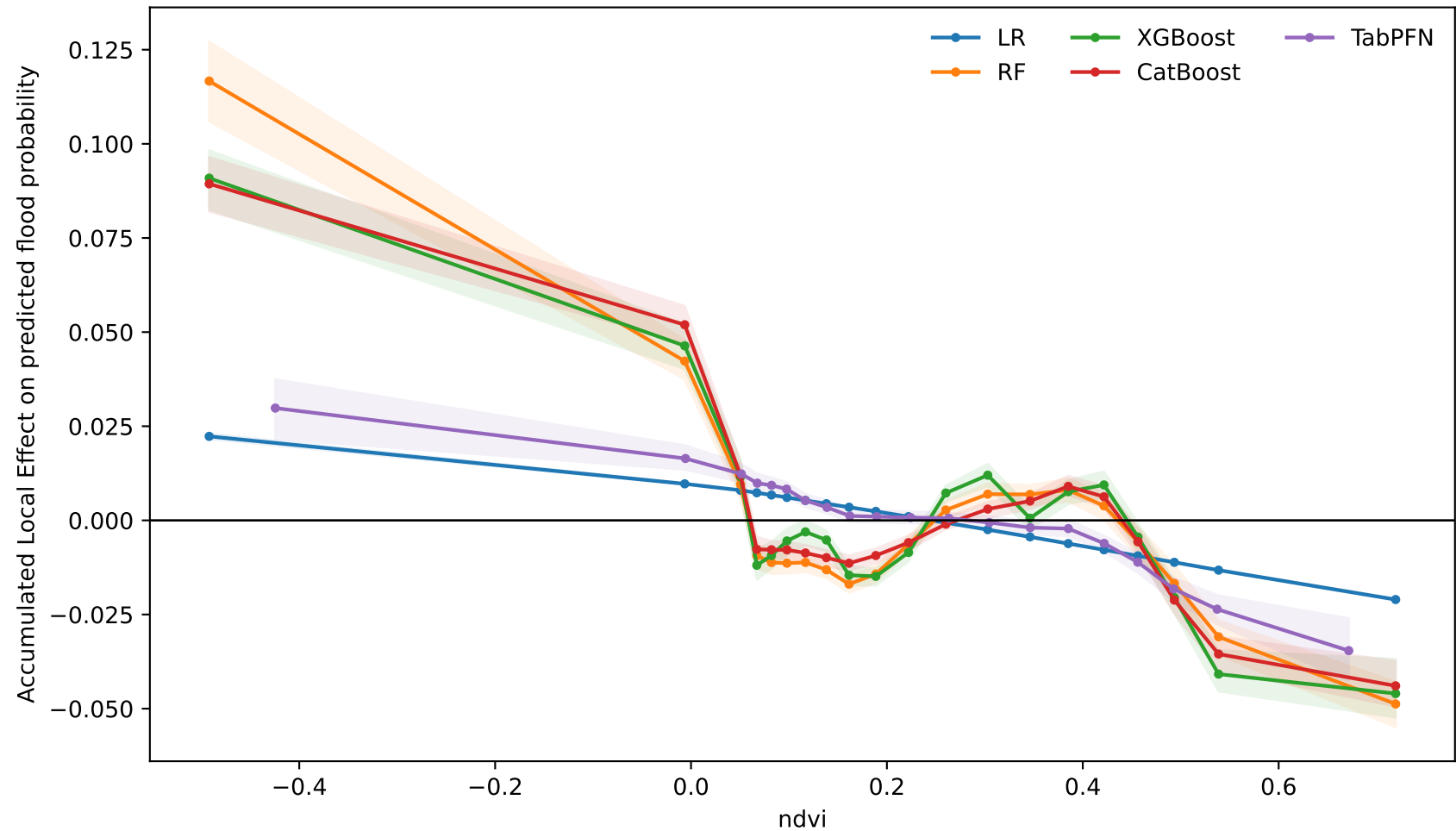
ALE comparison across five models — ndvi
