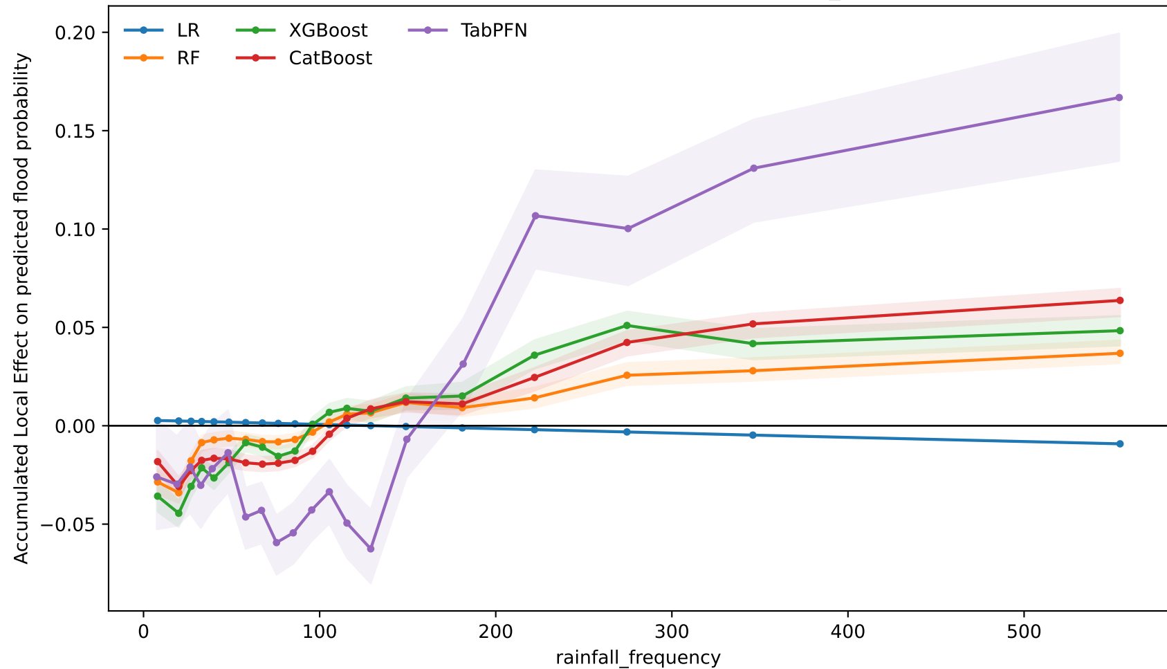
ALE comparison across five models — rainfall_frequency
