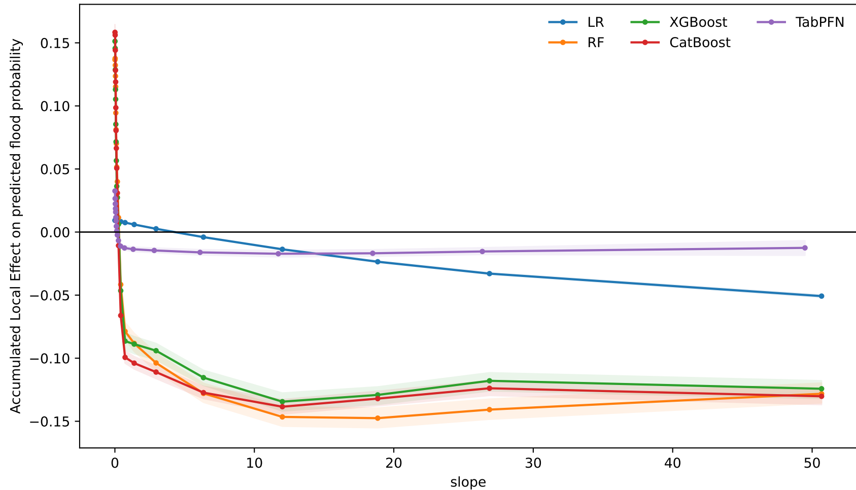
ALE comparison across five models — slope
