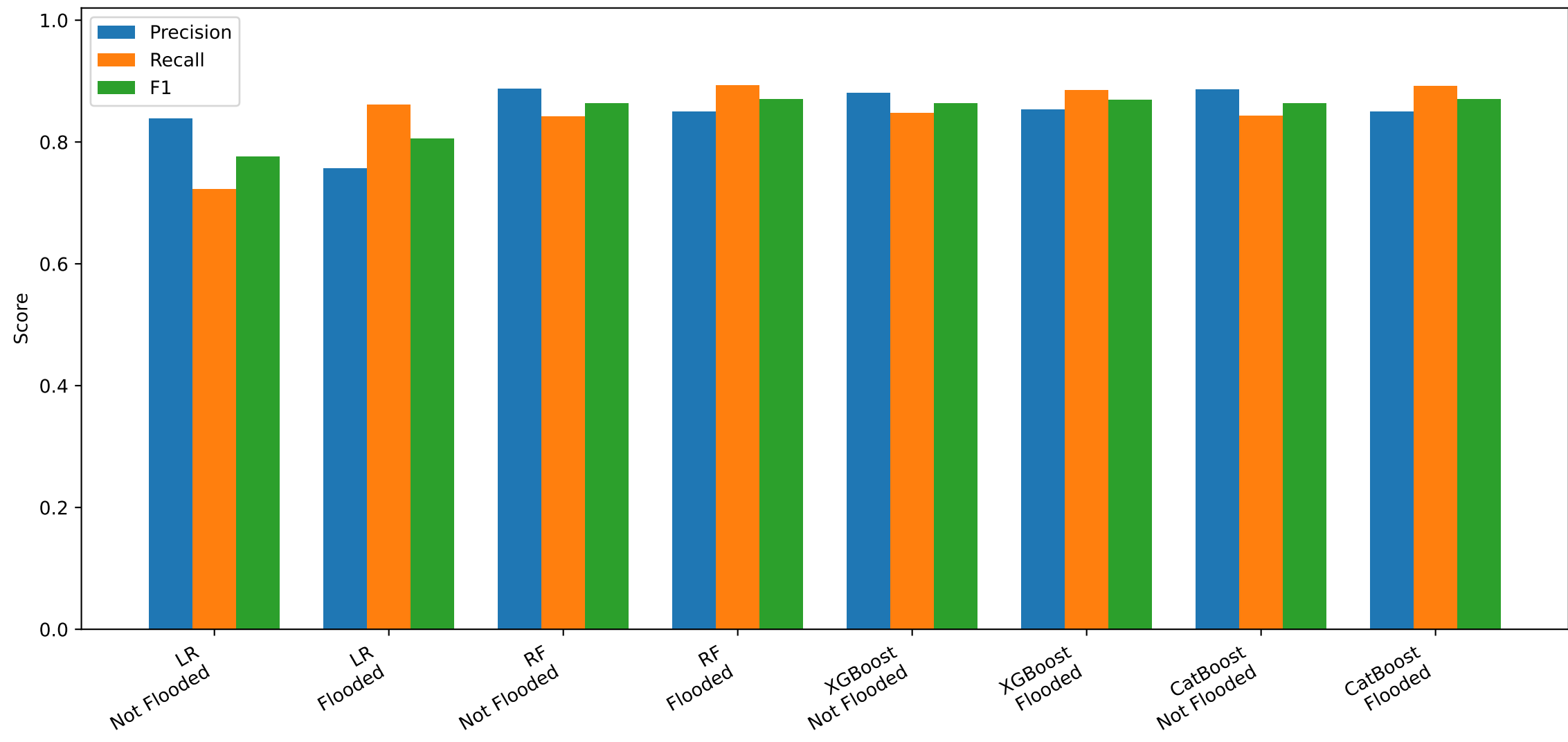
Class-wise Performance — Random Holdout
