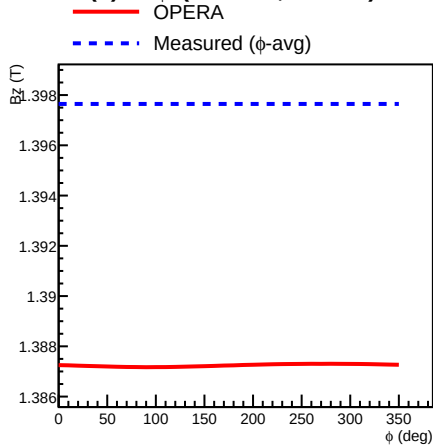
B_z (T) vs \phi (r=30 cm, z=0 cm)
