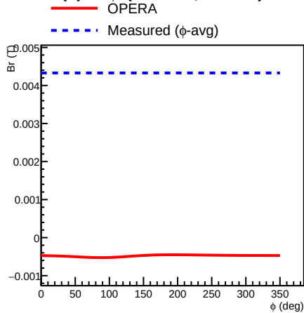
B_r (T) vs \phi (r=30 cm, z=0 cm)
