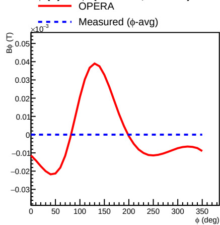
B_\phi (T) vs \phi (r=30 cm, z=0 cm)
