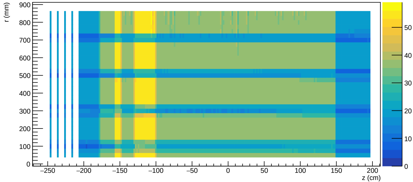
N(\phi) per (r,z) bin
