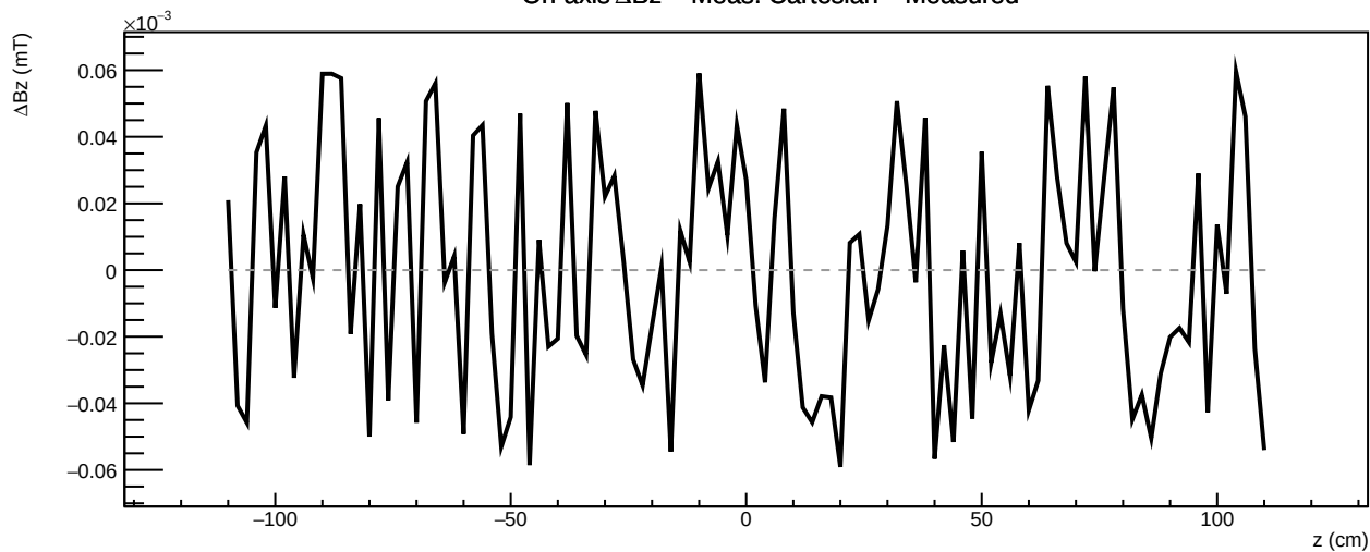
On-axis \Delta B_z = \text{Meas. Cartesian} - \text{Measured}
