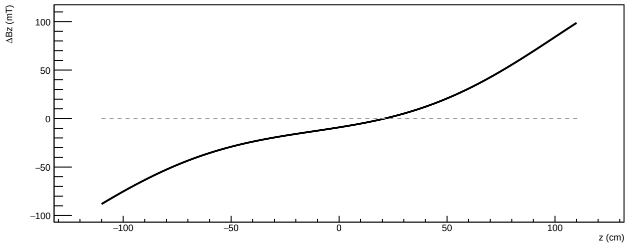
On-axis \Delta B_z = \text{Analysis} - \text{Measured}
