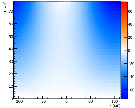
\Delta B_r (Analysis - Measured) [mT]
