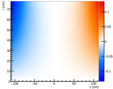
Analysis Br \phi -avg
