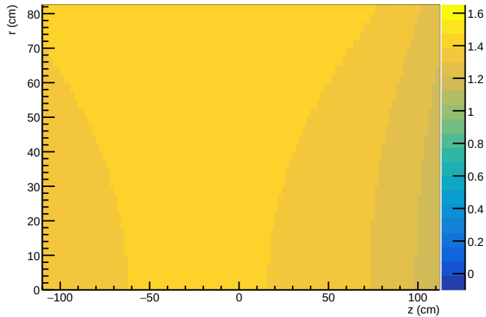
Meas. Cartesian Bz ( \phi -avg)
