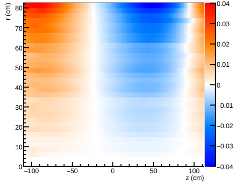
\Delta Br (Meas. Cartesian – Measured) [mT]
