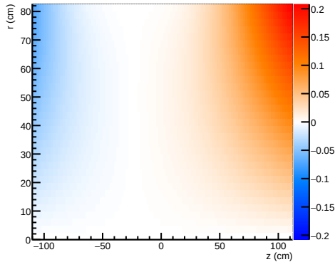
Meas. Cartesian Br ( \phi -avg)
