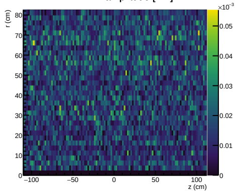
B_z m=1 amplitude [mT]
