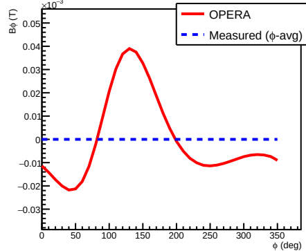
B \phi (T) vs \phi (r=30 cm, z=0 cm)
