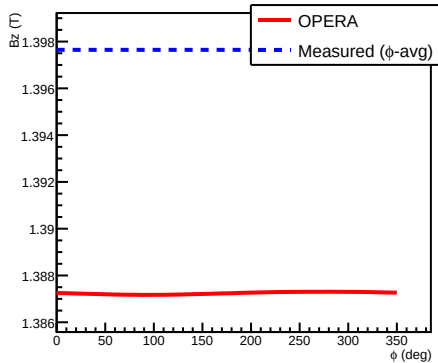
Bz (T) vs \phi (r=30 cm, z=0 cm)
