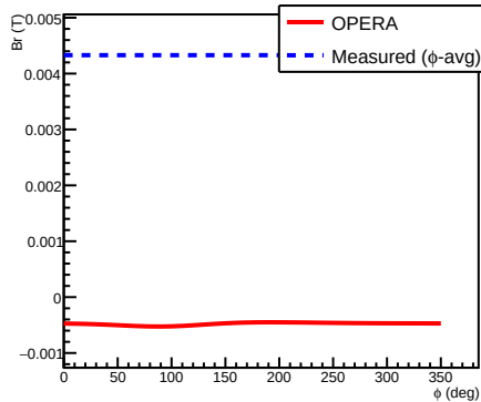
Br (T) vs \phi (r=30 cm, z=0 cm)
