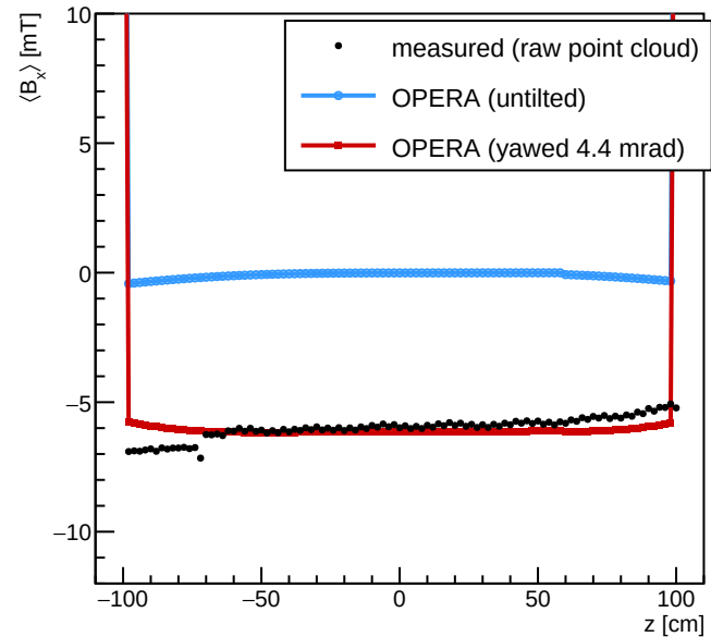
\langle B_x \rangle vs z (measured raw vs OPERA)
