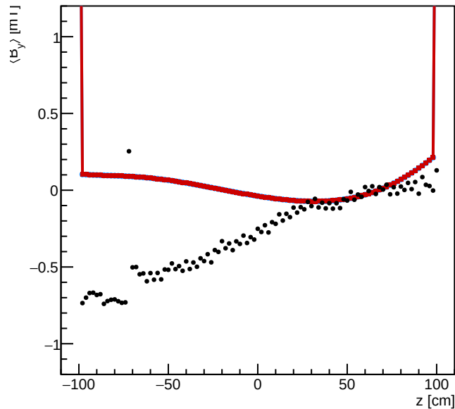
\langle B_y \rangle vs z (measured raw vs OPERA)
