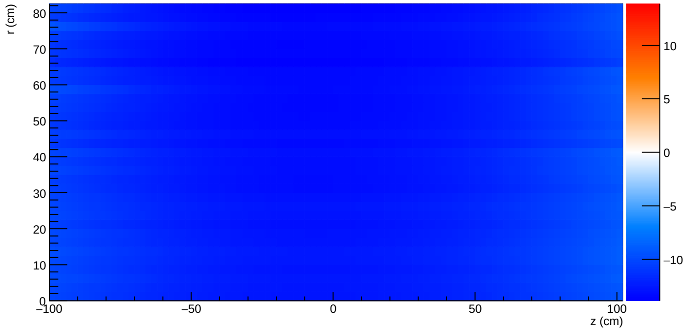
\Delta B_z (OPERA – Measured) [mT]
