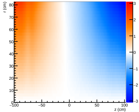
\Delta Br (OPERA - Measured) [mT]
