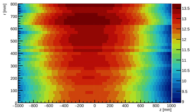
B_z measured - OPERA [mT]
