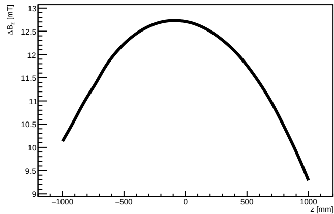
B_z measured - OPERA [mT]
