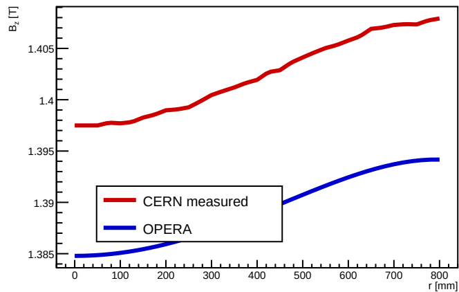
B_z vs r at z=0
