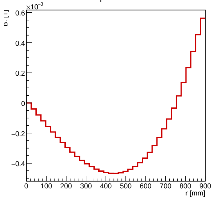
B_r at z = 0
