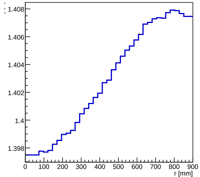
B_z at z = 0
