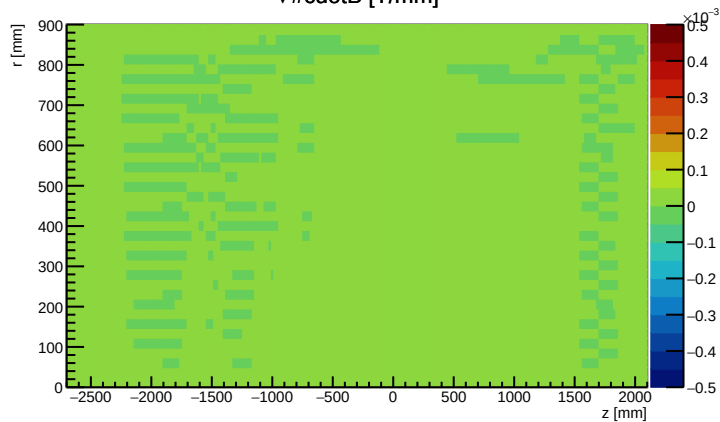
\nabla \cdot \mathbf{B} [T/mm]
