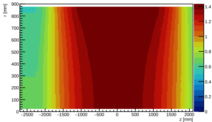
B_z [T] ( \phi -averaged, sPHENIX coords)
