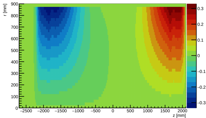
B_r [T] (Maxwell-consistent, from \nabla \cdot \mathbf{B} = 0 )
