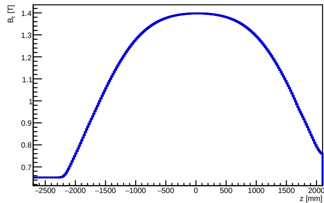
B_z on axis ( r = 0 )
