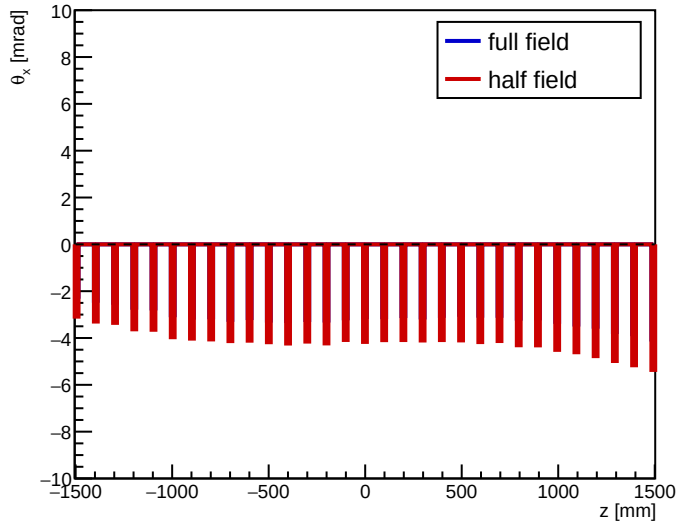
\theta_x(z) : full (blue) vs half (red) field
