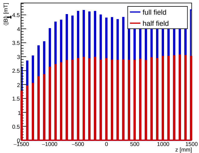
\langle |B| \rangle(z) : full (blue) vs half (red)
