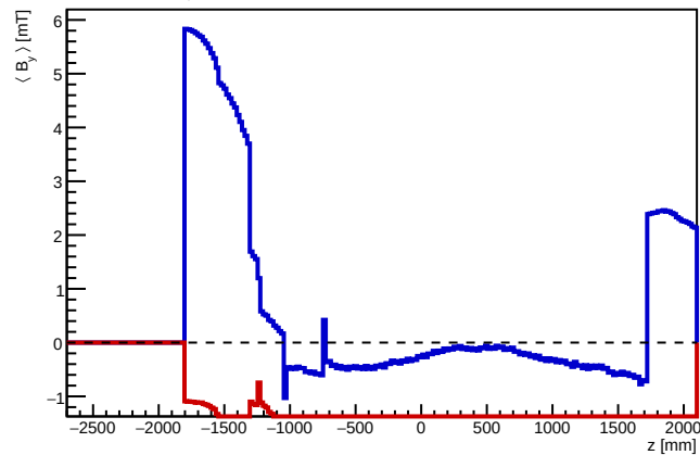
\langle B_y \rangle vs z (all r = blue, r < 150 mm = red)
