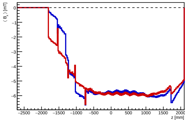
\langle B_x \rangle vs z (all r = blue, r < 150 mm = red)
