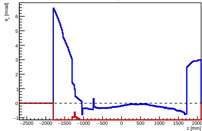
\theta_y = \text{atan2}(\langle B_y \rangle, \langle B_z \rangle)
