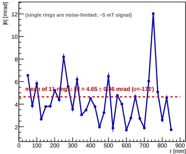
Method 1: |\theta|(r) per ring in central band ( |z| < 150 mm)
