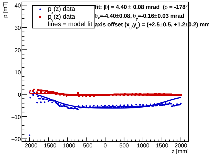
Method 2: transverse-field intercept p(z) (data) + model fit
