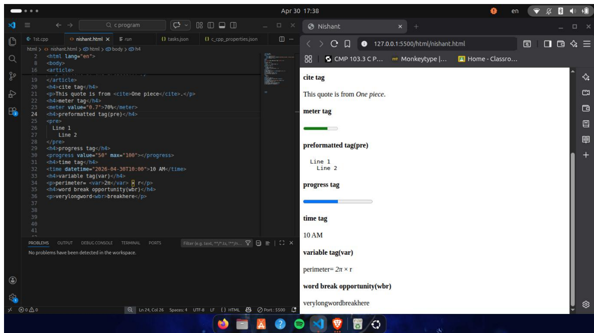
Fig:additional tag vs code
