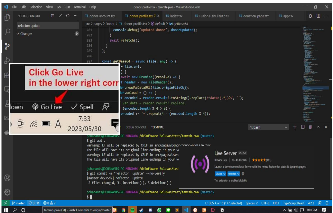
Fig:Live server and Vs code user interface
