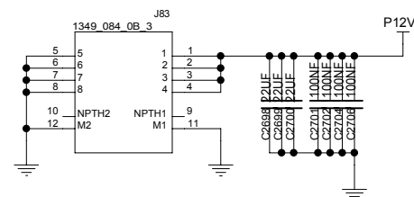
PWR_FOR_FRONT_BOARD
