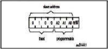
Figure 6. PCAN55 address
