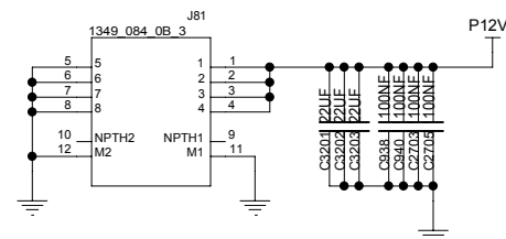
PWR_FOR_RISER_LEFT
