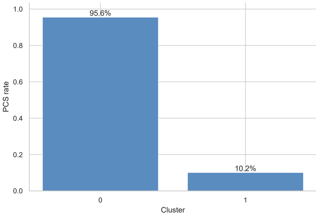
PCS occurrence rate by latent cluster
