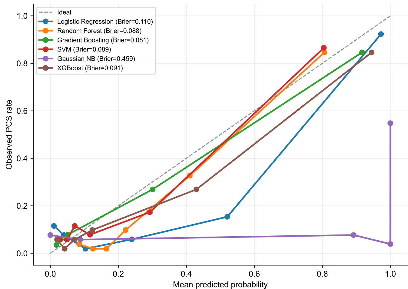
Cross-validated calibration curves
