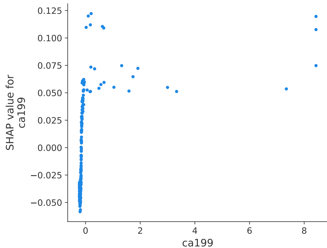
SHAP dependence: ca199
