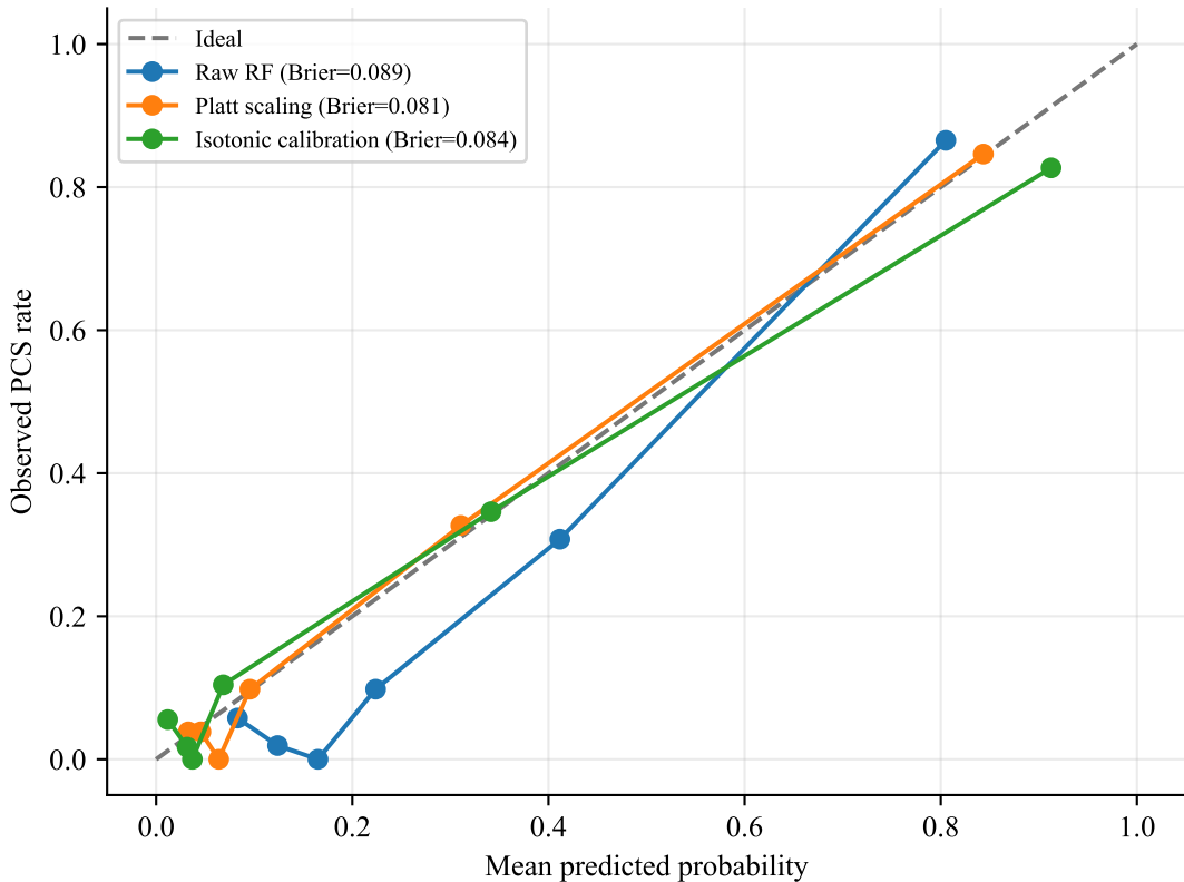
Calibration method comparison
