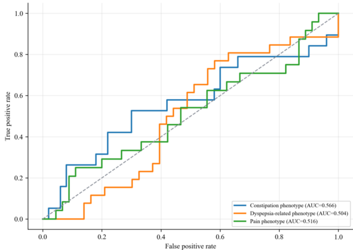
One-vs-rest ROC curves: XGBoost
