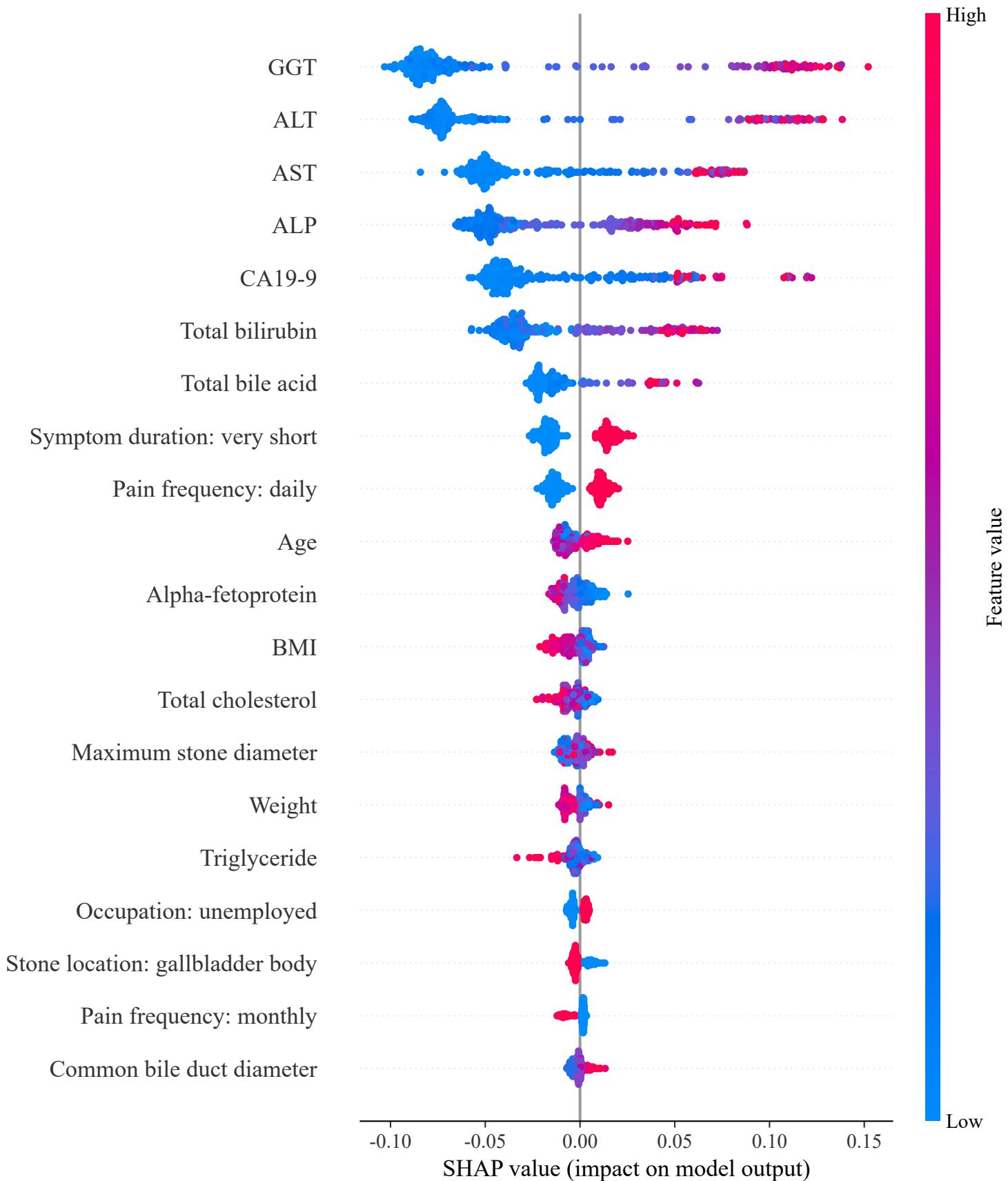
SHAP summary plot for PCS prediction
