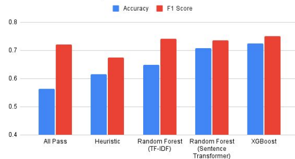
Evaluations: Accuracy and F1 Score
