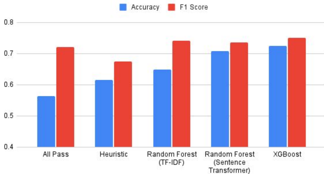
Evaluations: Accuracy and F1 Score
