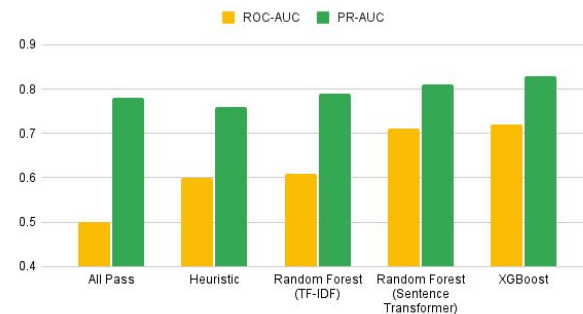
Evaluations: ROC-AUC and PR-AUC
