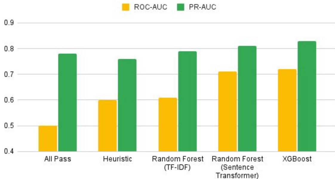
Evaluations: ROC-AUC and PR-AUC
