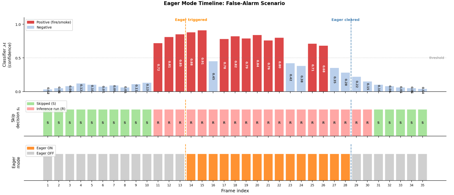
Figure 8: Per-frame timeline illustrating a false-alarm scenario under Eager mode. Once the classifier \mathcal{M} produces W_{\text{fire}} consecutive positive predictions on a static ambiguous scene, the system enters Eager mode (orange region), forcing inference on every subsequent frame and causing a sustained increase in FAR until W_{\text{clr}} consecutive negative predictions are observed.
