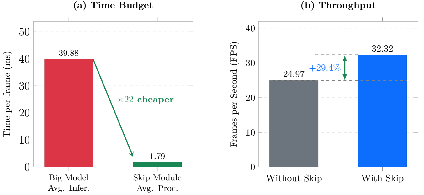
Figure 4: Computational efficiency of the proposed skip-module: (a) average processing time of the skip-module (1.79 ms) compared to the BIG model inference time (39.88 ms), representing a \times 22 reduction; (b) system throughput with and without the skip-module, yielding a 29.4% improvement in FPS.
