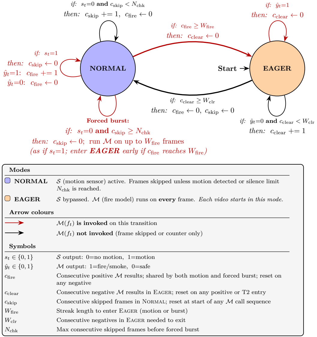
Figure 7: State machine of the eager mode extension to the ACCMOTIONDET-based skip module. Each transition is annotated with an if condition and a then action specifying variable updates. In NORMAL mode, \mathcal{S} gates inference: frames with no detected motion are skipped and c_{\text{skip}} is incremented until c_{\text{skip}} \geq N_{\text{chk}} , at which point a forced inference check is issued and c_{\text{skip}} is reset. When \mathcal{M} produces W_{\text{fire}} consecutive fire or smoke predictions ( c_{\text{fire}} \geq W_{\text{fire}} ), the system transitions to EAGER mode, where \mathcal{S} is bypassed and every frame is forwarded to \mathcal{M} to prevent missed detections during slow-developing or settling smoke events. The system returns to NORMAL mode only after W_{\text{clr}} consecutive negative predictions confirm that the scene is safe.
