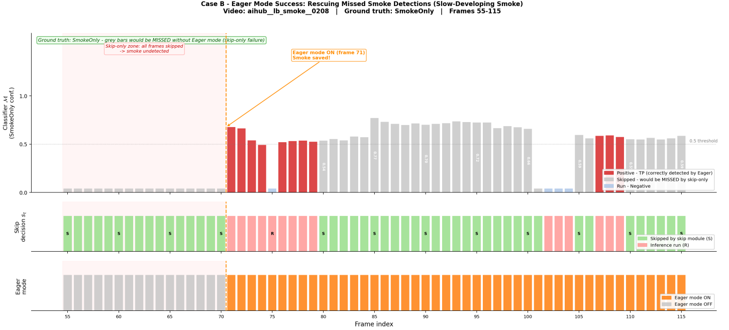
Figure 8: Per-frame timeline illustrating a successful recall-recovery scenario under Eager mode. The skip module initially suppresses inference on slow-developing smoke frames with minimal inter-frame motion (grey region). Once \mathcal{M} produces W_{\text{fire}} consecutive positive predictions on the first frames forwarded by the skip module, the system transitions into Eager mode (orange region), forcing inference on every subsequent frame and enabling continuous smoke detection that would otherwise have been missed by the skip module alone.
