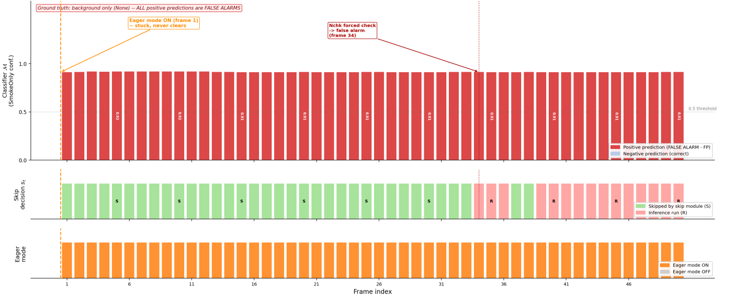
Figure 9: Per-frame timeline illustrating a false-alarm scenario under Eager mode. Once the classifier \mathcal{M} produces W_{\text{fire}} consecutive positive predictions on a static ambiguous scene, the system enters Eager mode (orange region), forcing inference on every subsequent frame and causing a sustained increase in FAR until W_{\text{clr}} consecutive negative predictions are observed.
