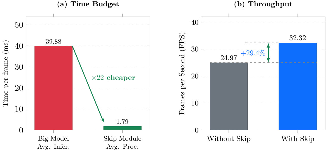
Figure 5: Computational efficiency of the proposed skip-module: (a) average processing time of the skip-module (1.79 ms) compared to the BIG model inference time (39.88 ms), representing a \times 22 reduction; (b) system throughput with and without the skip-module, yielding a 29.4% improvement in FPS.
