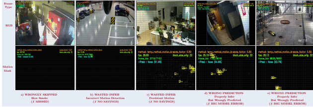
Figure 7: Qualitative analysis of skip module failure modes. (a) Missed detection: slow-developing or settled smoke fails to trigger the motion accumulator. (b–c) Wasted inferences: inaccurate motion detection or persistent motion (e.g., human activity) saturates the accumulator, preventing frame skipping. (d–e) Big Model error: frames are correctly passed to the deep learning model, yet the model produces incorrect predictions.
