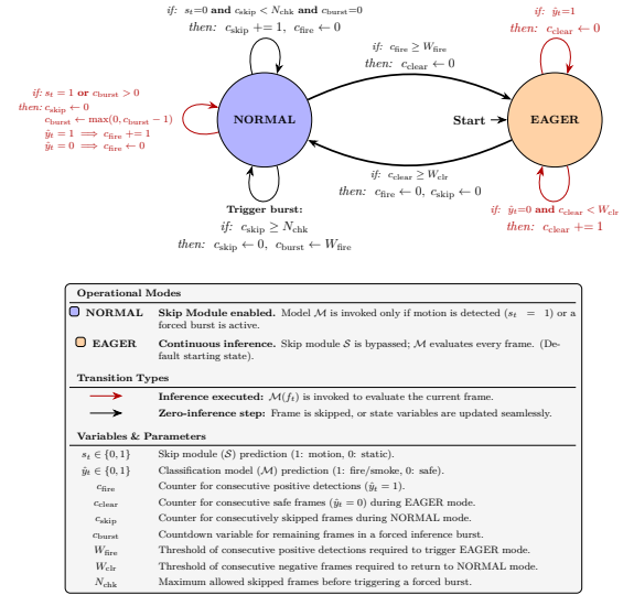
Figure 3: State machine of the EAGER mode extension to the AccMotionDet-based skip module. Transitions are annotated with if conditions and then actions specifying variable updates. In NORMAL mode, S operates as designed, with periodic forced checks every N_{\text{chk}} skipped frames. Upon W_{\text{fire}} consecutive positive predictions, the system enters EAGER mode, bypassing S (i.e., s_t = 1 ) to forward every frame to \mathcal{M} . The system returns to NORMAL mode after W_{\text{clr}} consecutive negative predictions.
