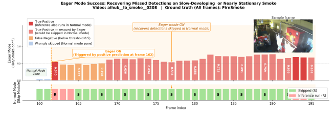
Figure 8: A per-frame timeline example illustrating a recall-recovery scenario under EAGER mode. Initially, the skip module suppresses inference on slow-developing smoke frames with minimal inter-frame motion (NORMAL Mode Zone). Once the classifier \mathcal{M} yields positive predictions on W_{\text{fire}} = 1 consecutive frame(s) in NORMAL mode, the system transitions to EAGER mode. This forces inference on every subsequent frame, enabling continuous smoke detection that would otherwise be missed—thus achieving a successful recall-recovery. Notably, from frames 163 to 168, the system returns None predictions yet remains in EAGER mode because the number of consecutive negative frames has not reached W_{\text{clr}} = 7 , which is insufficient to trigger an exit back to NORMAL mode.
