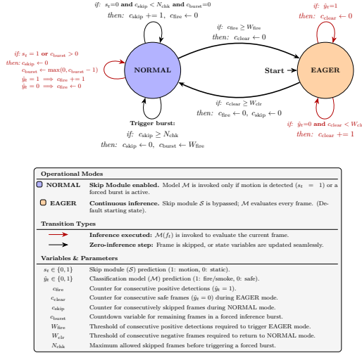
Figure 3. State machine of the EAGER mode extension to the AccMOTIONDET-based skip module. Transitions are annotated with if conditions and then actions specifying variable updates. In NORMAL mode, \mathcal{S} operates as designed, with periodic forced checks every N_{chk} skipped frames. Upon W_{fire} consecutive positive predictions, the system enters EAGER mode, bypassing \mathcal{S} (i.e., s_t = 1 ) to forward every frame to \mathcal{M} . The system returns to NORMAL mode after W_{clr} consecutive negative predictions.
