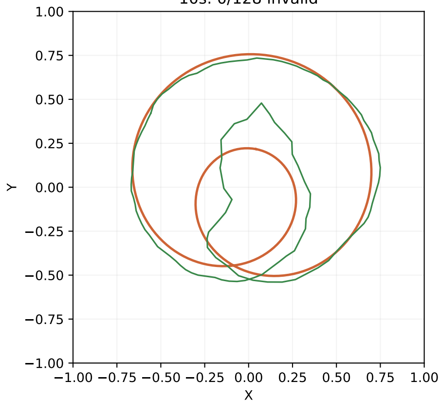
Gain corrected, alternative local solution 10s: 0/128 invalid
