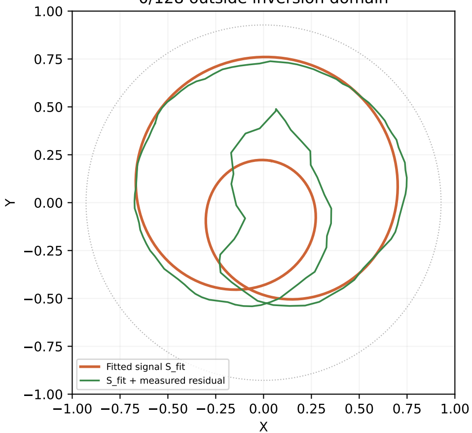
Alternative ( \sim 47\% BG) \cdot 10–11 s 0/128 outside inversion domain
