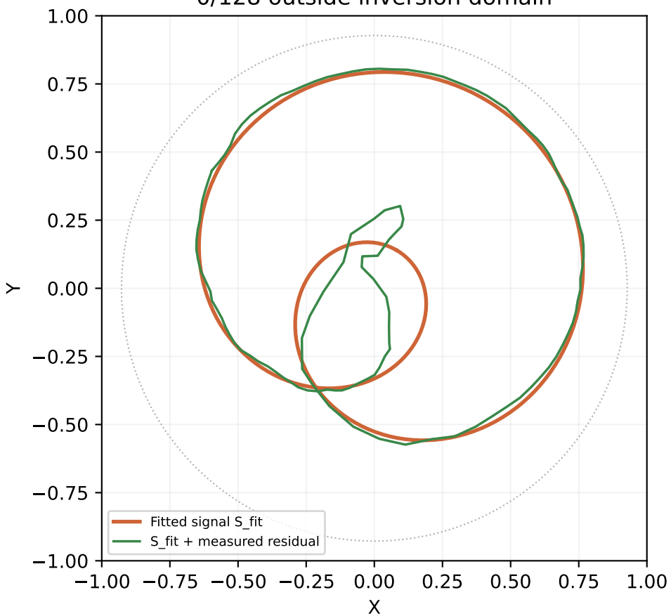
Alternative ( \sim 47\% BG) \cdot 30–31 s 0/128 outside inversion domain
