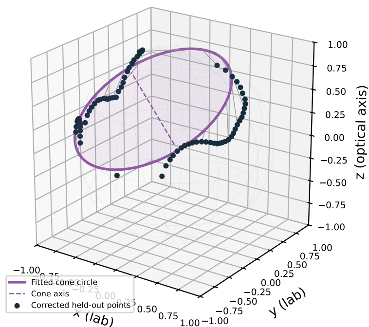
Unit sphere · 76/128 points invertible
