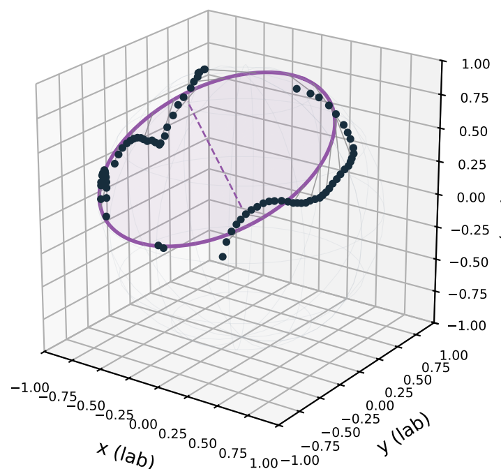
Unit sphere · 81/128 points invertible
