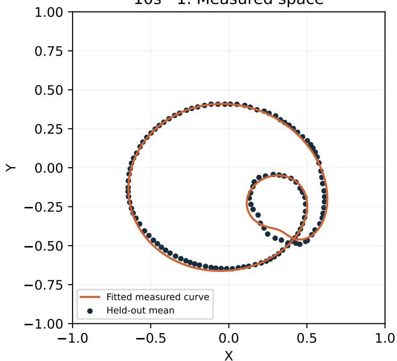
10s · 1. Measured space
