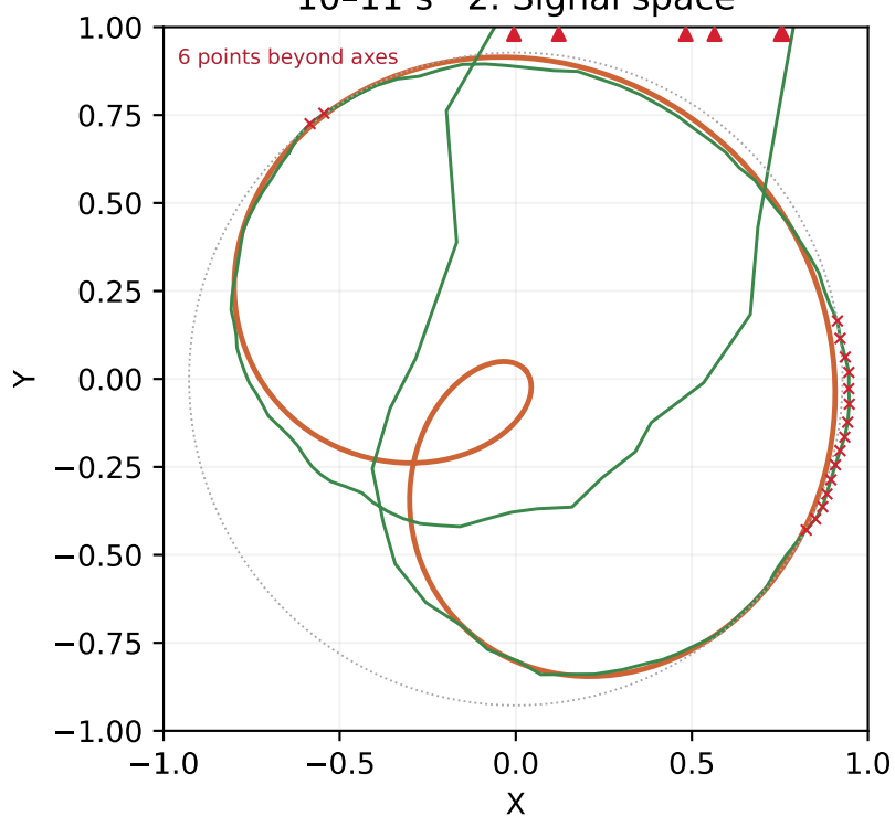
10-11 s · 2. Signal space
