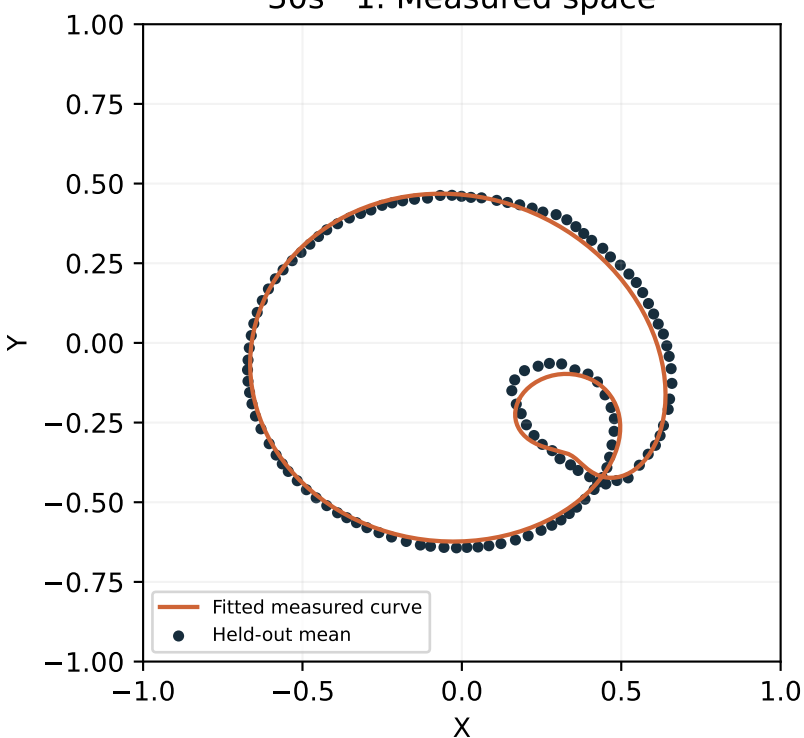
30s · 1. Measured space
