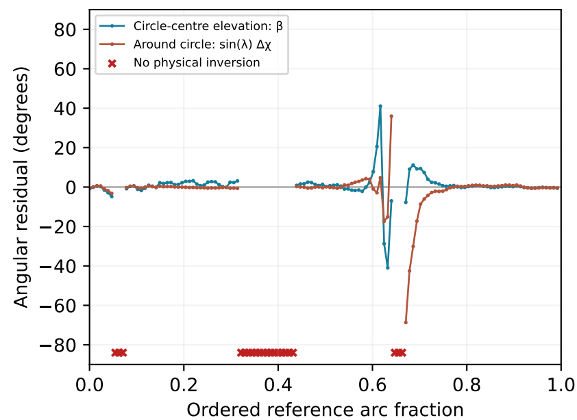
Residuals in fitted-cone frame
