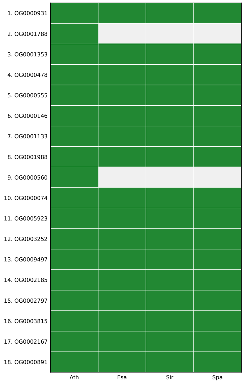
All 18 frozen orthogroups
