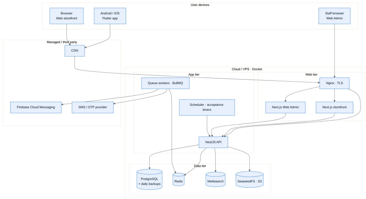
Figure 12. Deployment diagram — runtime infrastructure.
