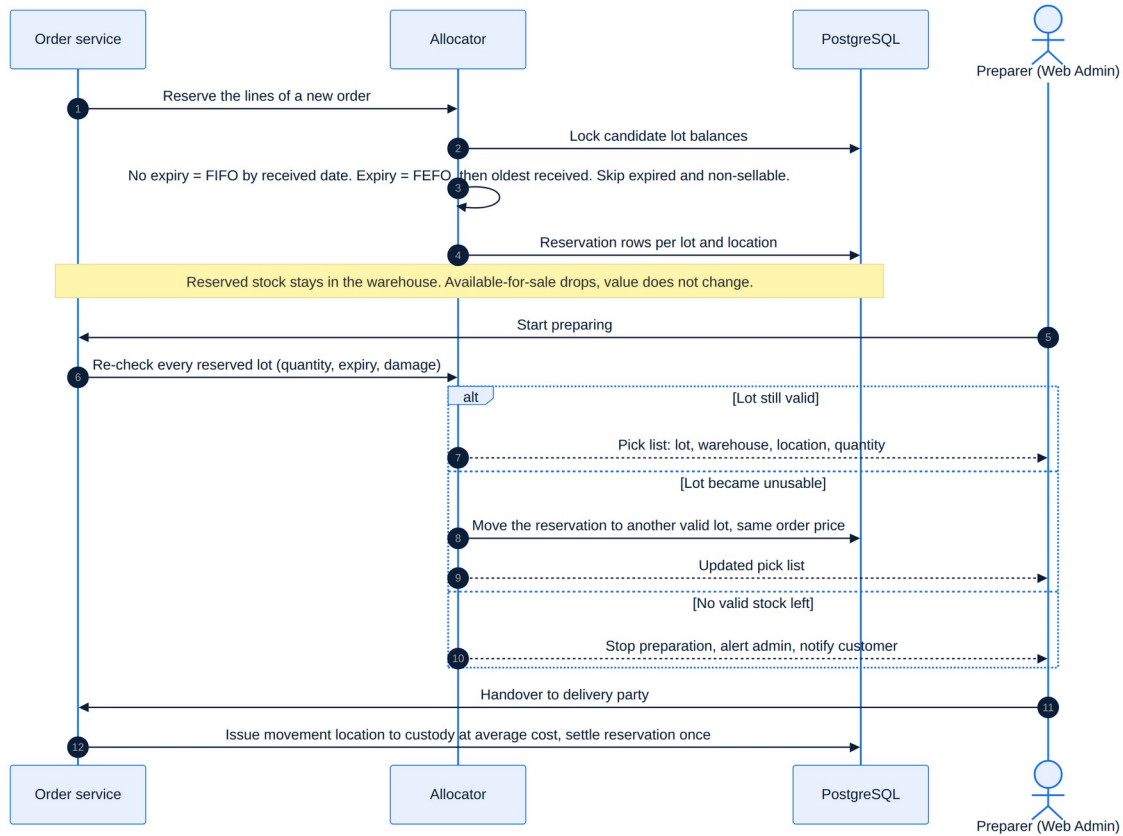
Figure 16. Sequence — allocation at order creation, re-check and reallocation at preparation, issue at handover.
