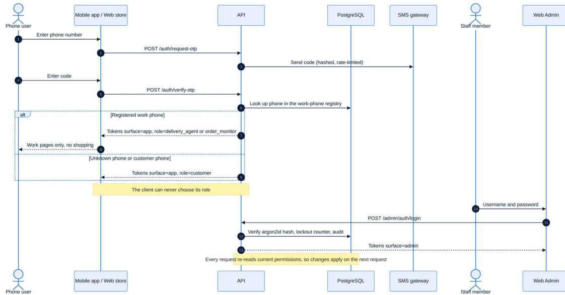
Figure 9. Sequence — OTP sign-in with server-assigned role, and Web Admin password login.
