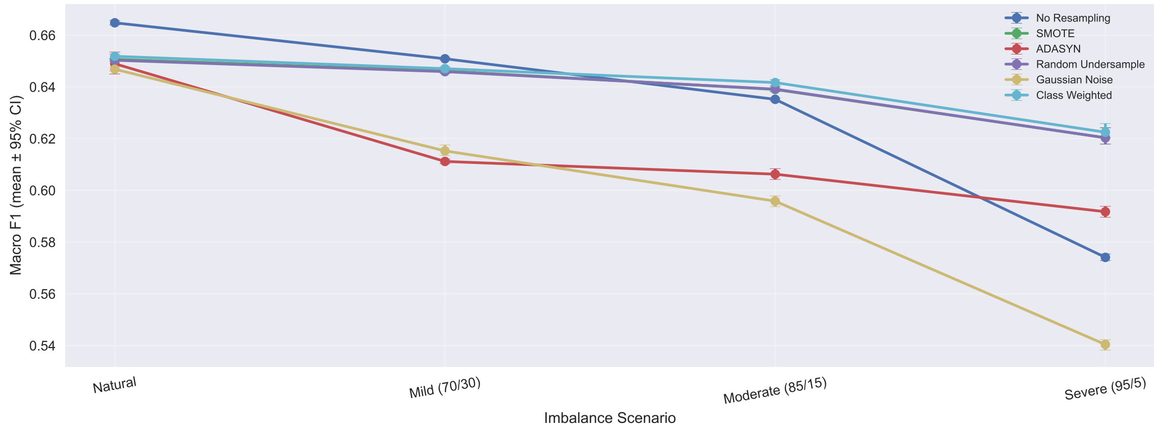
Figure 2: Macro-F1 Under Increasing Normal-Dominance Error bars = 95% bootstrap CI — XGBoost
